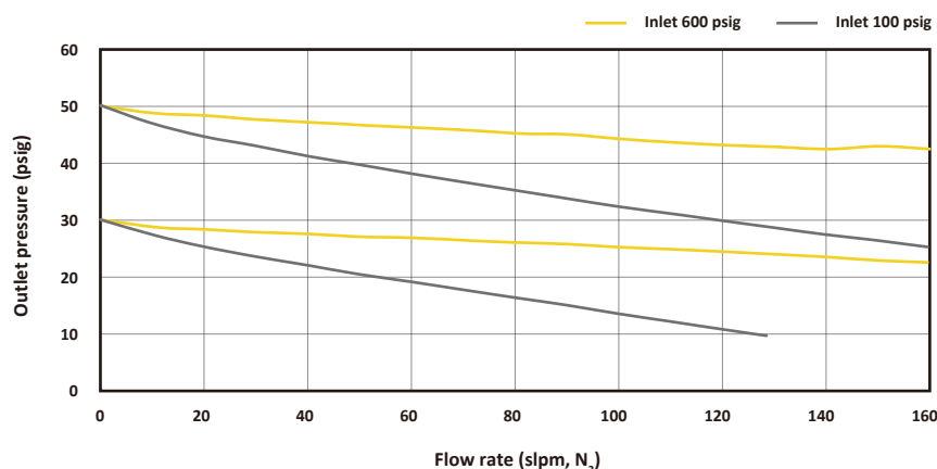
W1000 Flow curve
